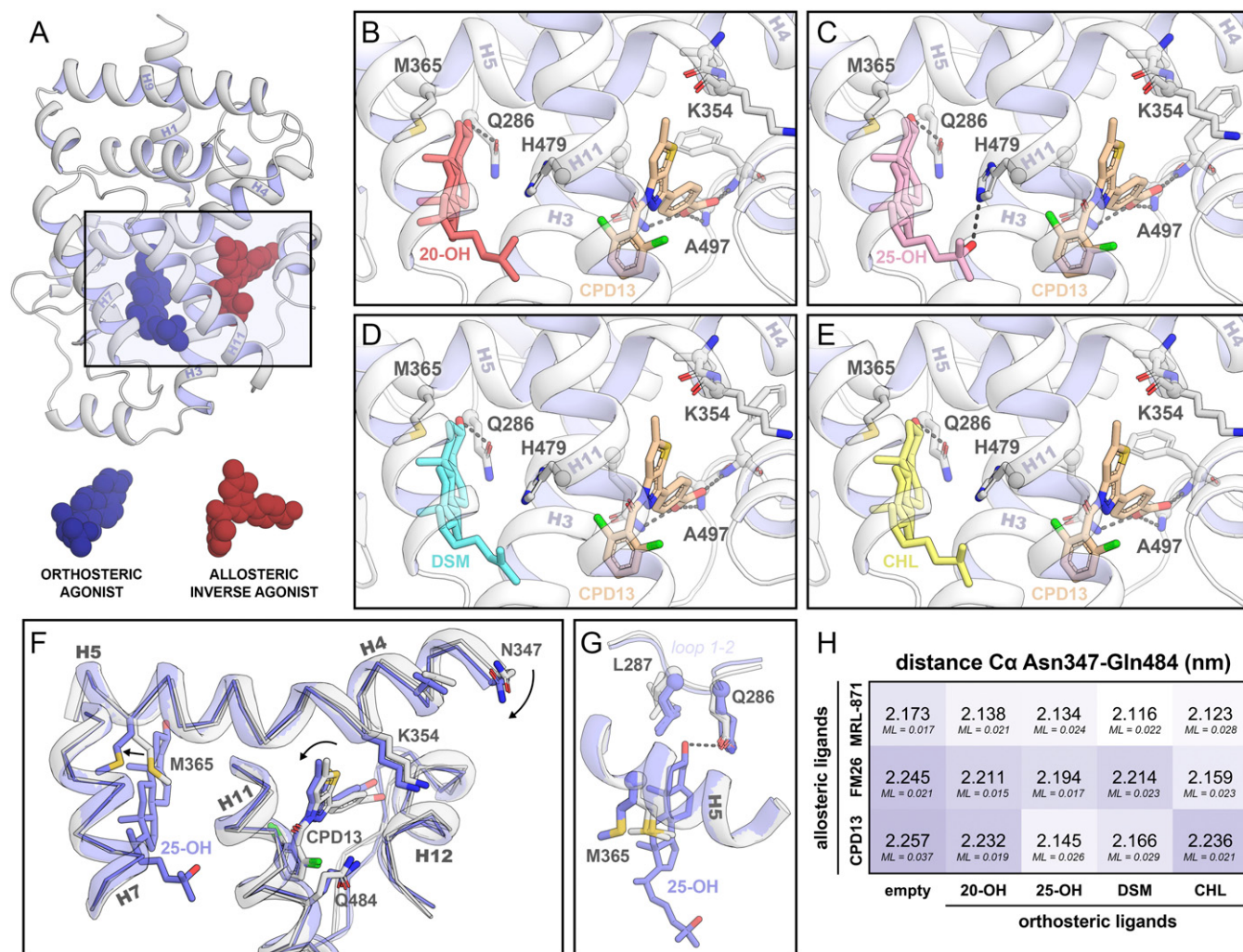
Fig. 4. Crystal structures of RORγt in complex with orthosteric and allosteric ligands. (A) Cartoon representation of RORγt in complex with an orthosteric (blue spheres) and an allosteric ligand (red spheres). The rectangle indicates the location of the zoomed-in orthosteric and allosteric LBP. (B–E) The orthosteric and allosteric LBP of RORγt in the presence of various orthosteric ligands (20-OH in red, 25-OH in pink, DSM in blue, and CHL in yellow) and the allosteric ligand compound 13 (brown). (F) Comparison of the crystal structures of RORγt in the presence (blue; PDB entry 6T50) or absence (white; PDB entry 6TLM) of an orthosteric modulator. The presence of the orthosteric modulator shifts helix 4 toward the allosteric pocket, thereby clamping the allosteric ligand. (G) Focused view of the orthosteric LBP. Side chains of Gln286, Leu287, and Met365 are shown for all crystal structures containing ligands in both pockets (12 structures in blue) as well as in absence of an orthosteric modulator (three structures in white; PDB entries 5C4O, 6SAL, and 6TLM). The presence of the orthosteric ligand locks Met365 into a defined state which is conserved for all 12 crystal structures containing orthosteric ligands. (H) Distance (in nm) between the α-carbons of Asn347 (helix 4) and Gln484 (helix 11) in the crystal structures. The maximum-likelihood coordinate error (ML; in nm) is provided for every structure.
