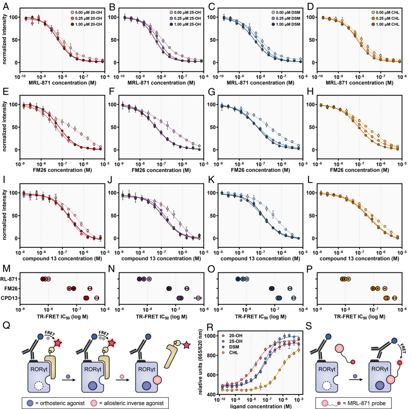
Fig. 3. (A–L) Dose–response curves of competitive TR-FRET coactivator recruitment assays by titration of allosteric ligands MRL-871 (A–D), FM26 (E–H), and compound 13 (I–L) to ROR \gamma t in the presence of fixed concentrations of 20-OH (A, E, and I), 25-OH (B, F, and J), DSM (C, G, and K), and CHL (D, H, and L) (0.00, 0.25, and 1.00 \mu M). The data were normalized with regards to plateau levels (nonnormalized data are provided in SI Appendix, Fig. S3 ). The data for FM26 were adapted from Meijer et al. (38). (M–P) Overview of the IC 50 values for MRL-871, FM26, and compound 13, at different fixed concentrations of the orthosteric ligands. The IC 50 values decreased as the concentration of orthosteric ligand increased. (Q) Schematic representation of the TR-FRET coactivator recruitment assay. When ROR \gamma t is in its apo or agonist-bound state, the cofactor binds to the LBD, resulting in FRET pairing from an anti-His terbium cryptate donor to the D2-labeled streptavidin (binding to biotin-labeled cofactor). (R) Dose–response curves of a TR-FRET assay with an AlexaFluor647-MRL-871 allosteric probe, by titration of the orthosteric ligands 20-OH, 25-OH, DSM, and CHL to a fixed concentration of ROR \gamma t (20 nM) and allosteric MRL-871 probe (100 nM). (S) Schematic representation of the TR-FRET assay using the AlexaFluor647-labeled MRL-871 probe. When the probe binds to the ROR \gamma t LBD, fluorescence emission occurs via FRET pairing between an anti-His terbium cryptate donor and the probe. Data are recorded in triplicate from three independent experiments (one representative dataset shown). Error bars represent the SD of the mean.
