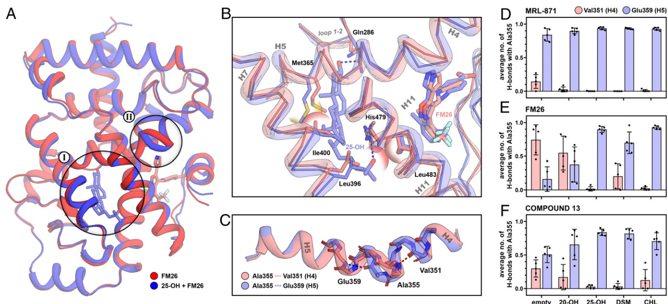
Fig. 5. Comparison of the RORyt complexes bound to an allosteric ligand in the presence (blue) or absence (red) of an orthosteric ligand using MD. (A) Superposition of the average structure of FM26 with and without 25-OH. The orthosteric LBP (I) and the transition between helices 4 and 5 of RORyt (II) are highlighted. (B) Focused view of the orthosteric LBP of RORyt. Polar interactions are shown as dashed lines, and steric clashes are shown as semitransparent spheres. (C) Isolated helices 4 and 5 showing the conformational switch of Ala355 from helix 4 to 5 upon orthosteric ligand binding. (D–F) The average number of hydrogen bonds of Ala355 with Val351 (helix 4; red) or Glu359 (helix 5; blue) in the presence of different orthosteric and allosteric modulators over the course of the simulation. Bars represent the average value over five independent simulations with the individual values represented as black spheres and the error bar showing the SD.
