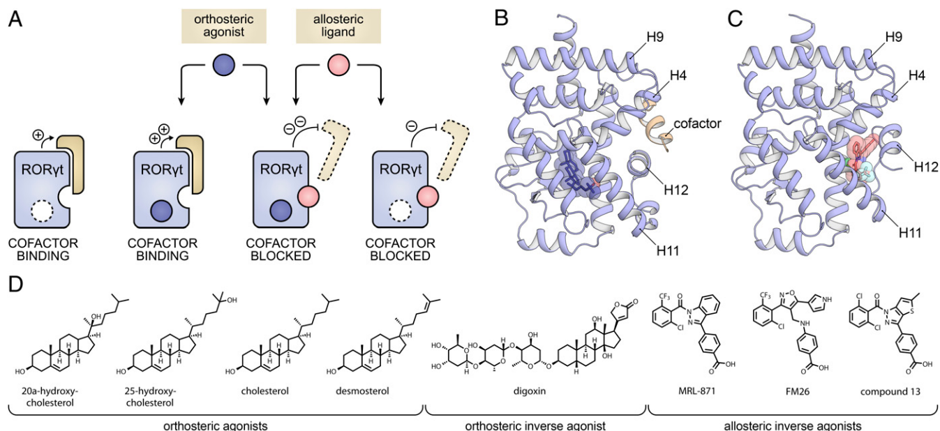
Fig. 1. (A) Conceptual representation of the ROR \gamma t LBD which is intrinsically active in the apo state, inducing cofactor binding. In the presence of an orthosteric agonist (blue), cofactor binding is further increased, while in the presence of an allosteric inverse agonist (pink), cofactor binding is blocked. In the presence of both an orthosteric and an allosteric ligand, the cofactor blockage is most efficient because of cooperative dual ligand binding. (B) Crystal structure of the ROR \gamma t LBD with the agonist 25-OH bound to the orthosteric site (blue sticks; PDB entry 3L0L). (C) Crystal structure of the ROR \gamma t LBD with inverse agonist MRL-871 bound to the allosteric site (red sticks; PDB entry 5C4O). The structures show that the orthosteric and allosteric binding sites do not overlap and highlight the prominently different orientation of H12. (D) Chemical structures of ROR \gamma t orthosteric agonists (20-OH, 25-OH, CHL, and DSM), orthosteric inverse agonist (digoxin), and allosteric inverse agonists (MRL-871, FM26, and compound 13) used in this study.
