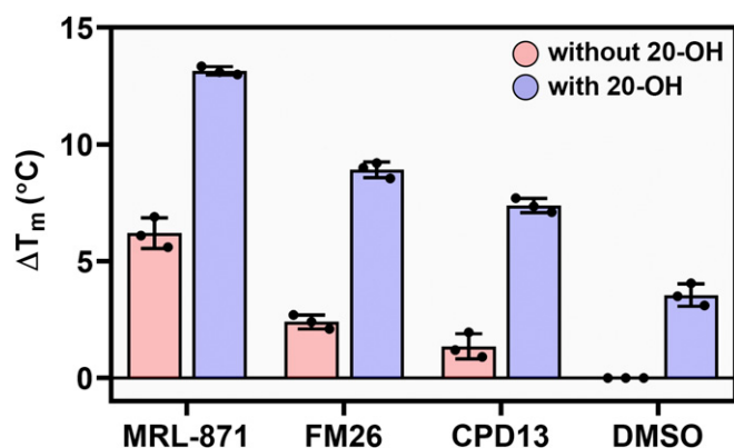
Fig. 2. Thermal stability of ROR \gamma t (5 \mu M) using a TSA format in presence of allosteric ligands MRL-871 (15 \mu M), FM26 (60 \mu M), and compound 13 (20 \mu M) (lowest concentrations giving a maximal \Delta T_m so maximal binding) as well as DMSO, in the absence (blue bars) and presence (pink bars) of 20-OH (60 \mu M). Data are recorded in triplicate from three independent experiments. Data are presented as mean \Delta T_m (normalized to DMSO) \pm SD.
